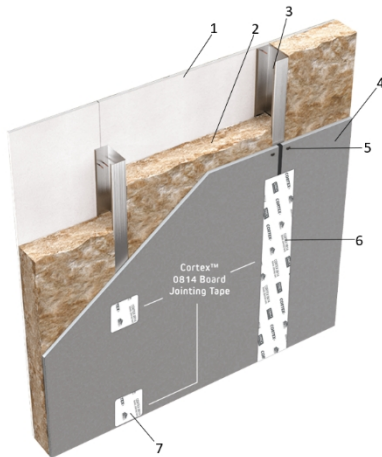
Diagram 1 - typical construction detail with tape
