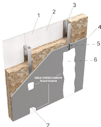
Diagram 3 - Typical construction detail with board sealant
