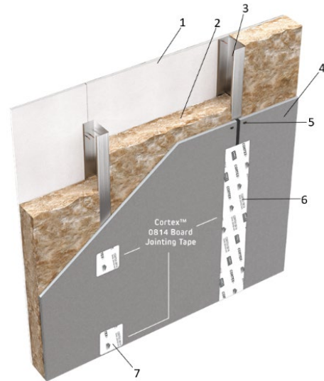
Diagram 2 - Typical construction detail with tape
